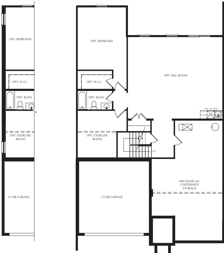
Partial foundation plan with left side end villa
