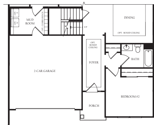
Partial main level with slab condition
