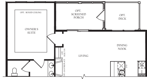
Partial main level with opt. Screened Porch
